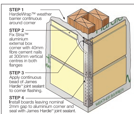
FIGURE 14 STRIA 14MM EXTERNAL BOX CORNER - STANDARD AND WIDE PROFILES
